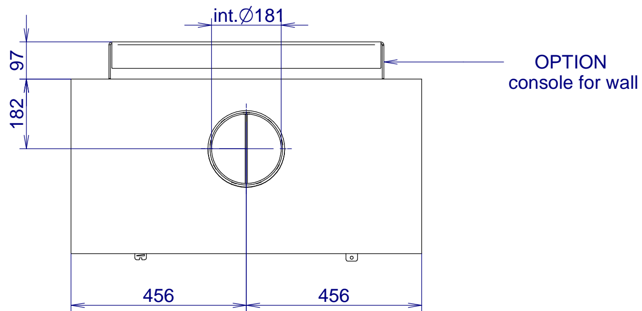
VENUS 850 V24 in the box + console for wall
